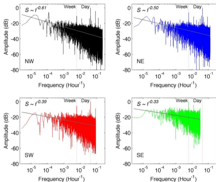
Figure 2. Lomb-Scargle Spectra corresponding to the four wind sectors. The following parameters were used hifac=1 (that defines the frequency limit as hifac times the average Nyquist frequency), ofac=4 (oversampling factor). This exponent, ( n -exponent) is defined from the asymptotic spectral amplitude, S , with the frequency, f , usually written as S \sim f^{-n} .
