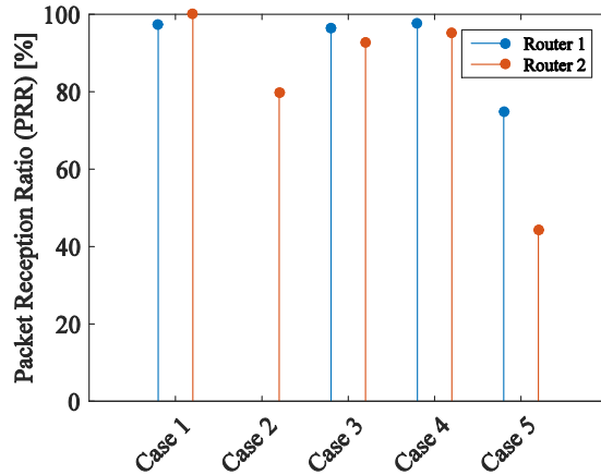
Figure 20. Graphical comparison of the five cases tested in case study A
