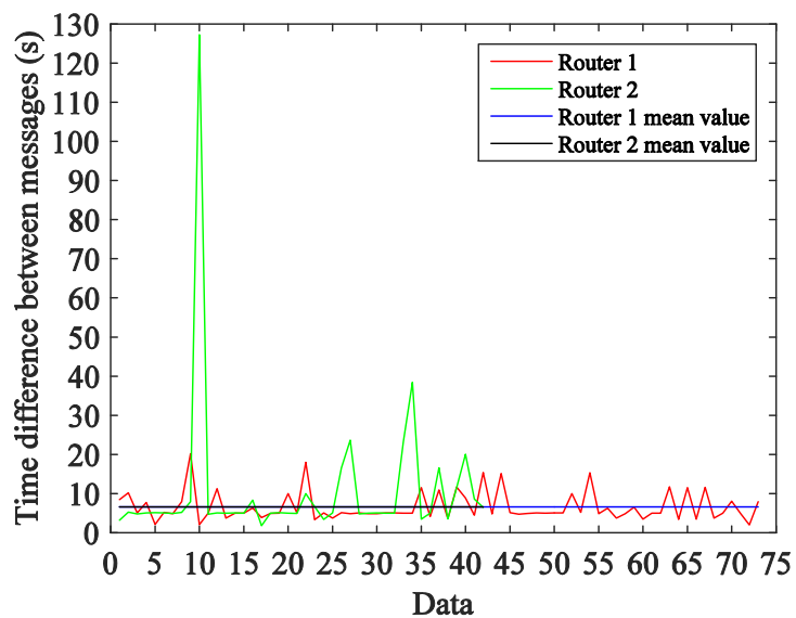
Figure 19. Case A.5: Time intervals between the data points received.
