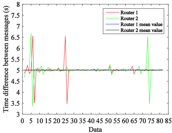
Figure 18. Case A.4: Time intervals between the data points received.
