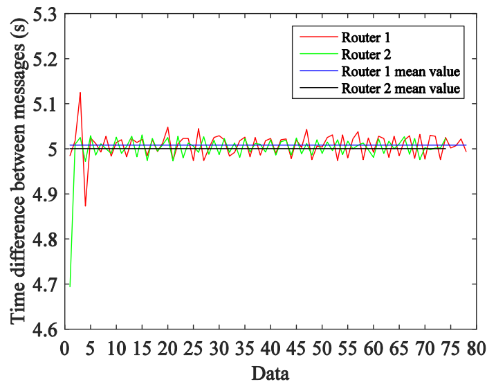
Figure 17. Case A.3: Time intervals between the data points received without the initial points.
