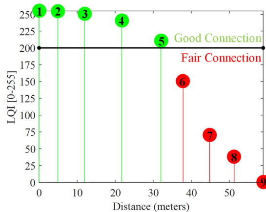
Figure 22. Graphical comparison of all Link Quality Indicator (LQI) values acquired in test 4.3.
