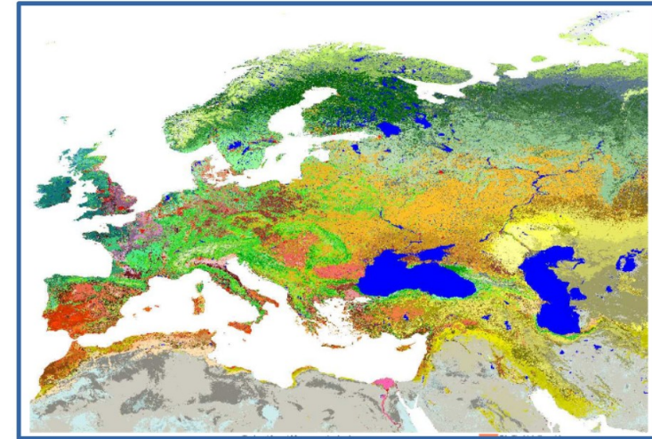
Ecoclimap-II map over Europe Faroux et al., 2013
