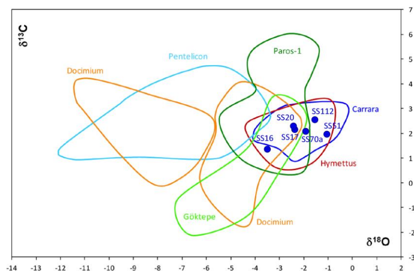
Figure 10. Isotopic signature of SS16, SS17, SS20, SS51, SS70a, and SS112 samples, compared with the reference database (after Antonelli and Lazzarini, 2015) for white marbles with MGS < 2 mm.
