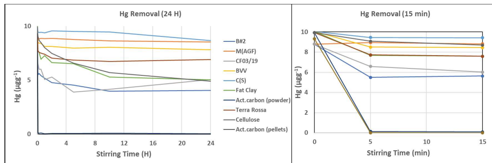
Figure 2 Hg removal from the mine water, by nature and waste products
