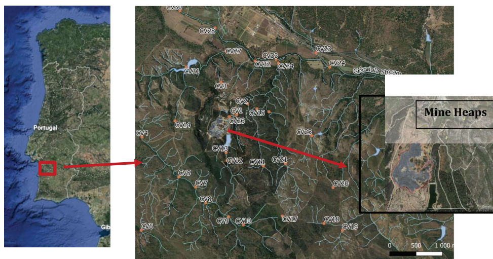
Figure 1. Location of the mine heaps of Caverna and sampling design in the watercourses affected by the AMD.
